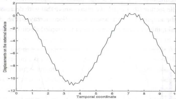
FIGURE 5 Time-dependency of displacements on the external surface of the cylinder (radial preliminary polarization; thickness l=0.13 )
