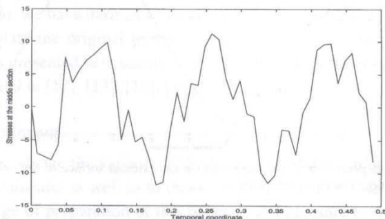
FIGURE 4 Time-dependency of stresses in the middle section of the cylinder (radial preliminary polarization; thickness l = 0.08 )
