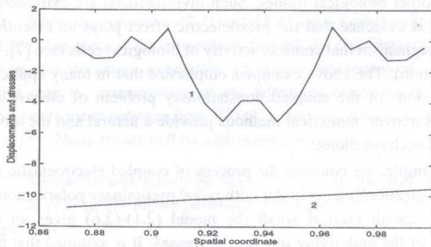
FIGURE 1 Radical stresses (curve 1) and displacements (curve 2) at t = 10 (radial preliminary polarisation ; thickness l = 0.13 )
