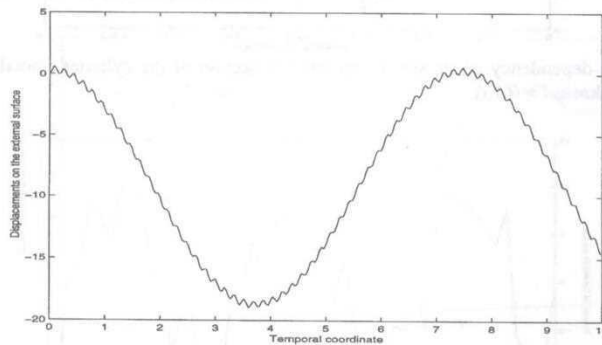
FIGURE 6 Time-dependency of displacements on the external surface of the cylinder (radial preliminary polarization; thickness l = 0.08 )
