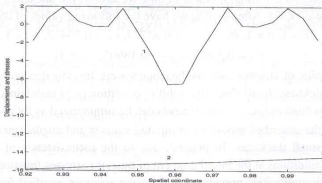
FIGURE 2 Radical stresses (curve 1) and displacements (curve 2) at t = 10 (radial preliminary polarisation ; thickness l = 0.08 )
