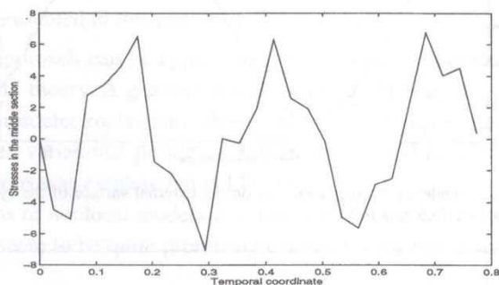
FIGURE 3 Time-dependency of stresses in the middle section of the cylinder (radial preliminary polarization; thickness l = 0.13 )
